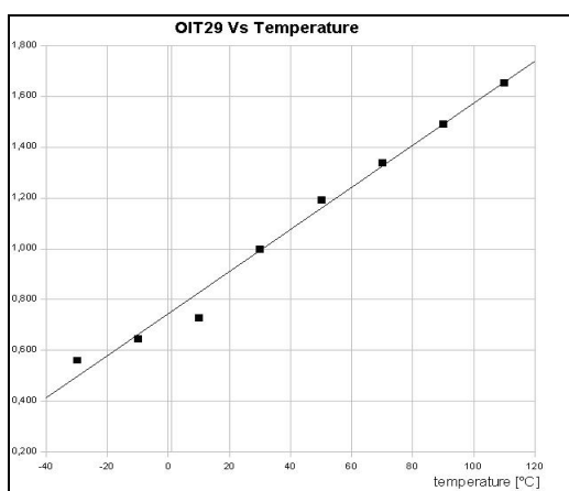
Figure 1 – Output voltage Vs Temperature
