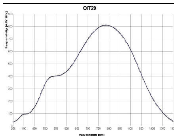
Figure 2 – Spectral Responsivity (h fe =1000)
